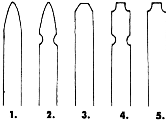
DOWELED END CONSTRUCTION
